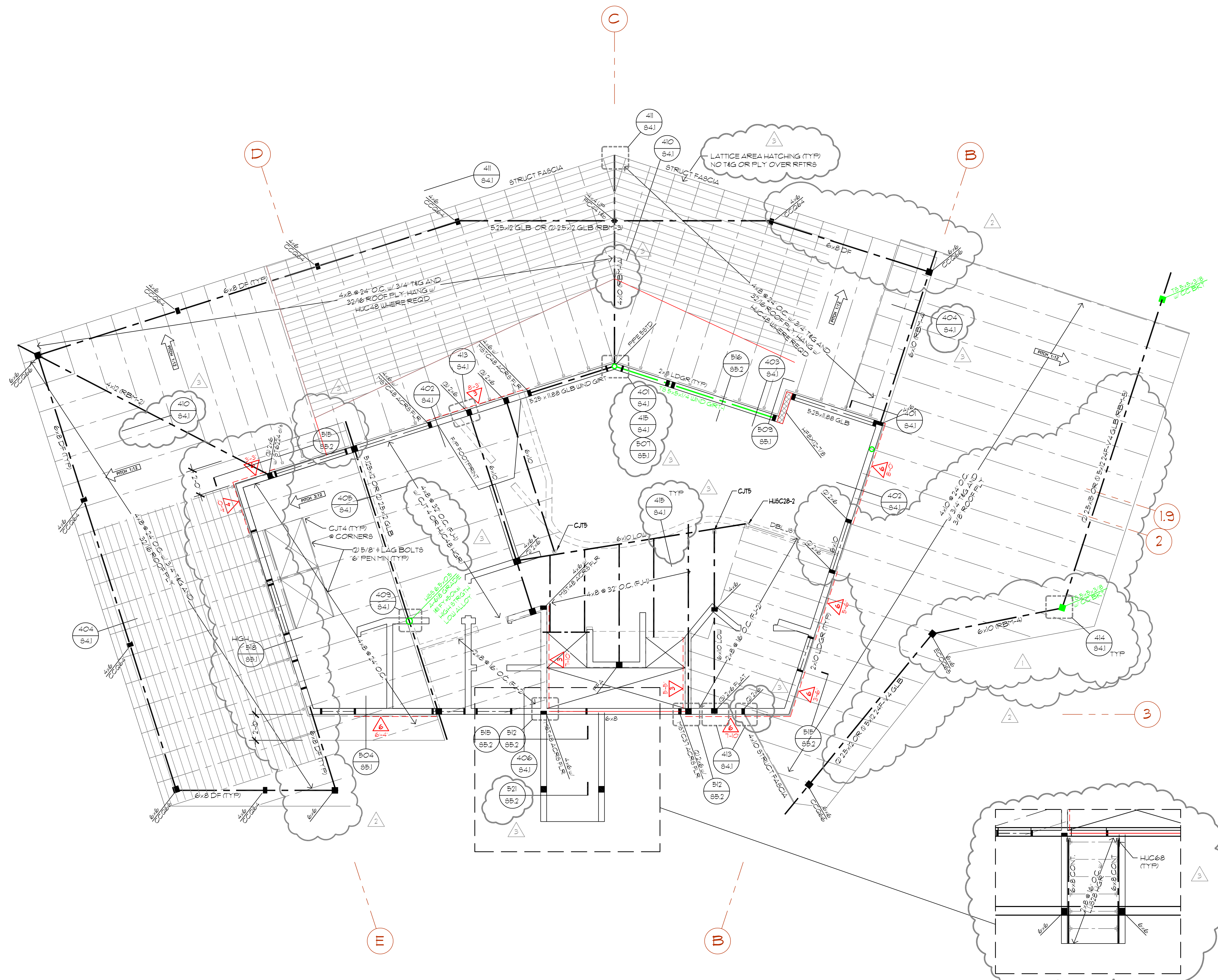
UPPER LEVEL FLOOR & LOWER LEVEL ROOF FRAMING SCALE: 1/4" = 1'-0"
